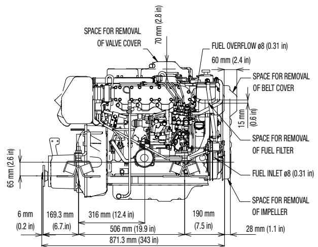
4JH5E with KM35P marine gear
