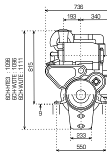
Engine only / Front view
